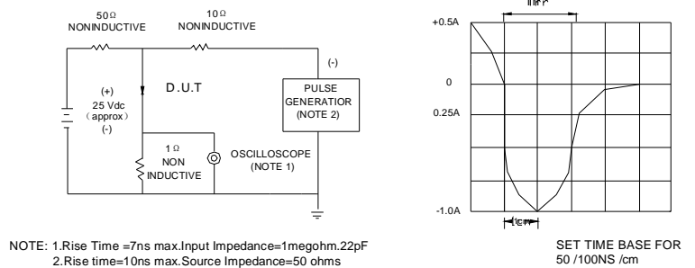
FIG.6-TEST CIRCUIT DIAGRAM AND REVERSE RECOVERY TIME CHARACTERISTIC
