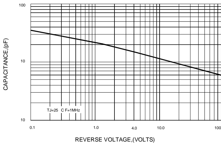
FIG.5-TYPICAL JUNCTION CAPACITANCE
