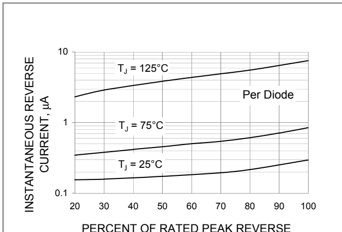
Fig.3- TYPICAL REVERSE CHARACTERISTIC
