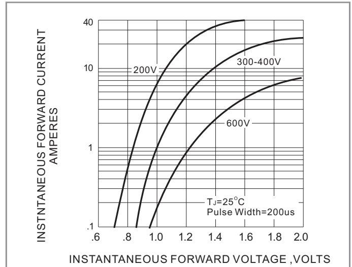
Fig.4- TYPICAL INSTANTANEOUS FORWARD CHARACTERISTIC
